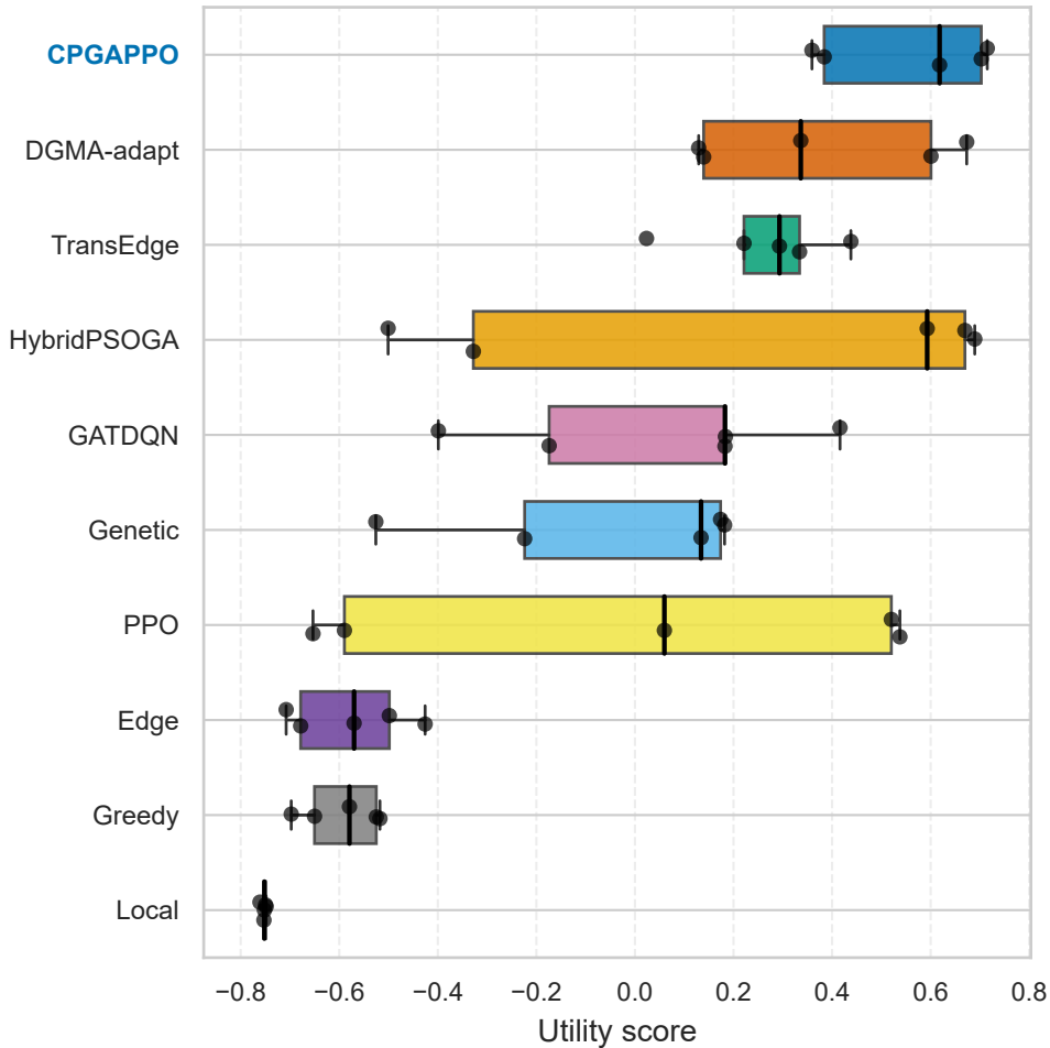
UtilityScore (per-seed cross-DAG avg, median + IQR, n=5 seeds)
